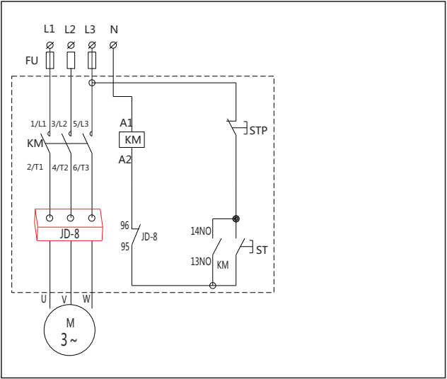
b. Connection diagram of NJBK5-10D in case the main circuit voltage is AC380V and the control circuit voltage is AC220V
